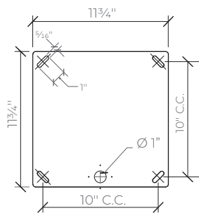
3/16" THICK SLIP-ON MOUNTING PLATE TOP VIEW SCALE: N.T.S.
